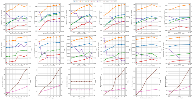
Fig. 8. Quantitative ablation on the number of prototypes v , prompts p , sparsity of frequency decomposition, the number of experts n and activated experts k , the minimum and maximum rank combination, and the corresponding computation and model complexity.
